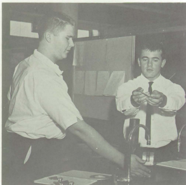
Curtis Carmack and Tony Goodpaster conduct an experiment demonstrating the law that like magnetic poles repel each other.
